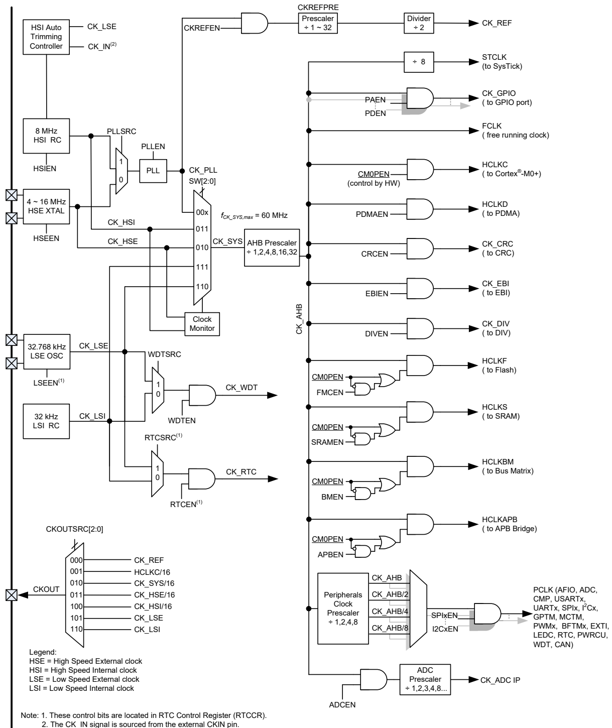
Figure 4. Clock Structure
