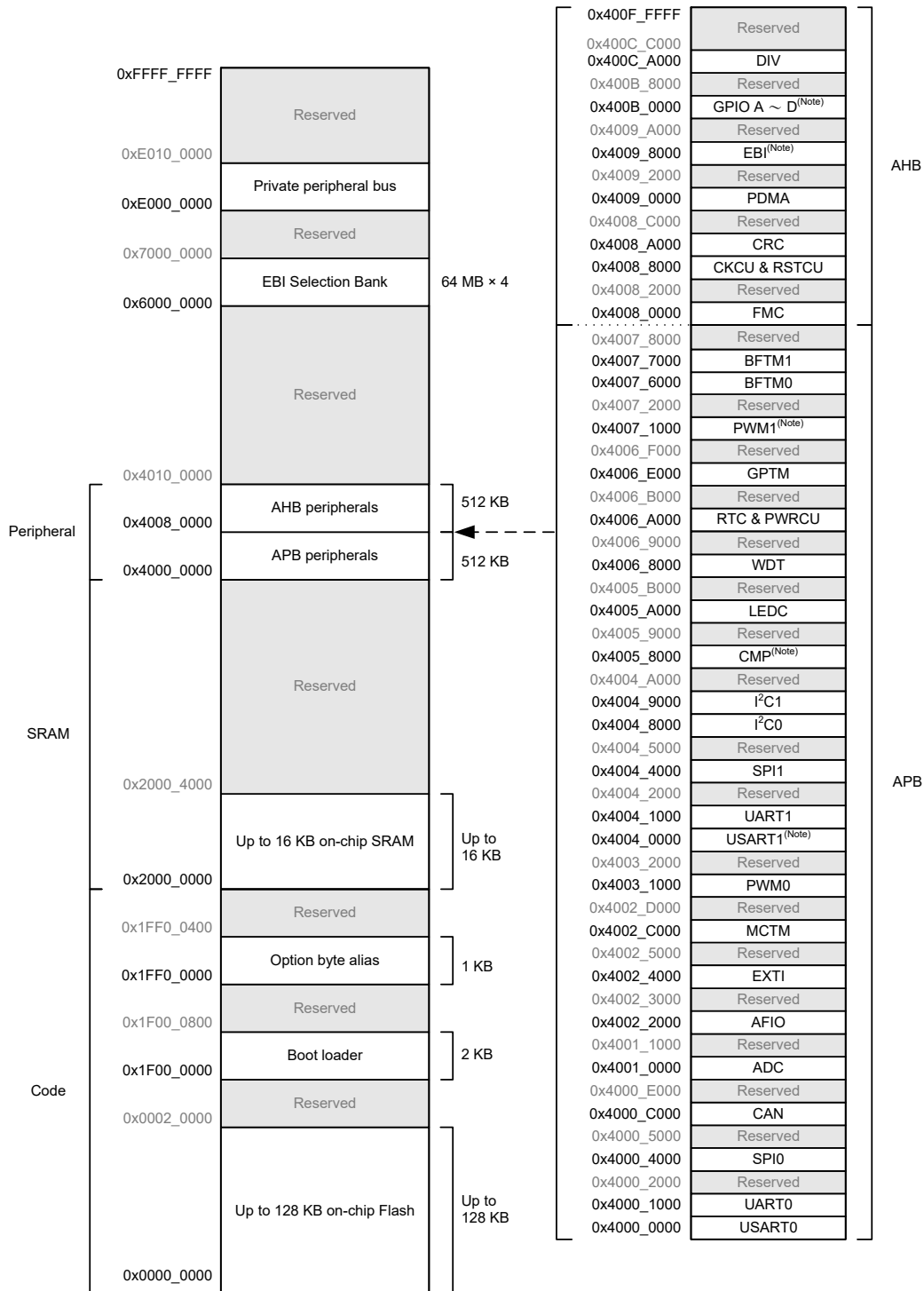
Figure 3. Memory Map
