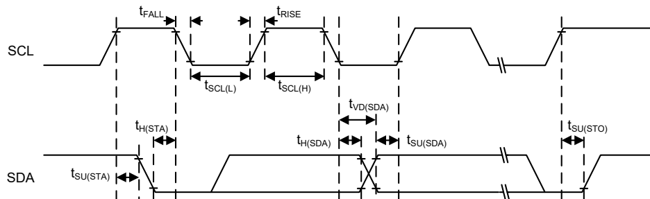
Figure 13. I 2 C Timing Diagram
