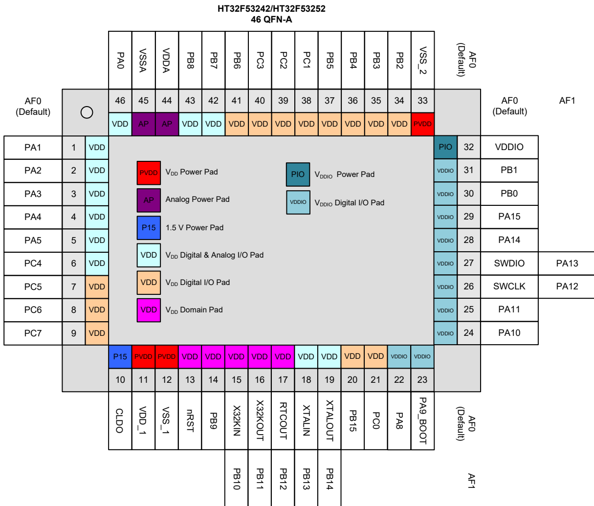
Figure 6. HT32F53242/HT32F53252 46-pin QFN Pin Assignment
