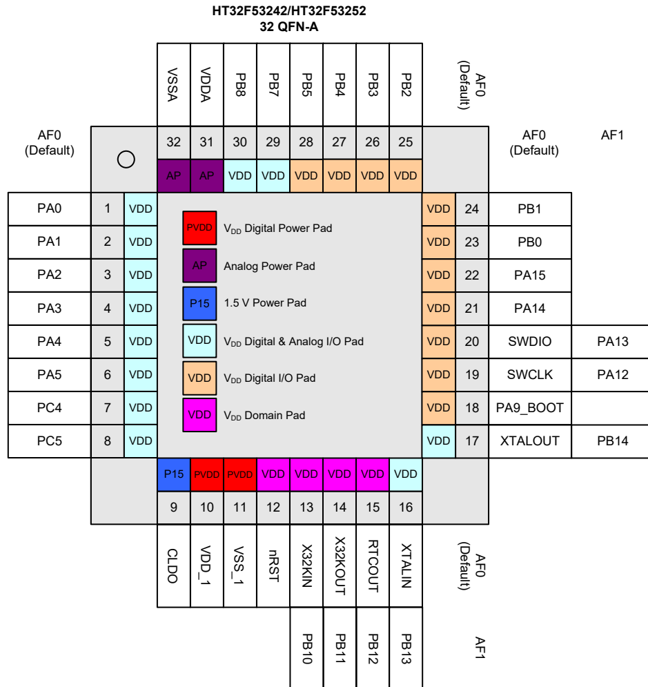
Figure 5. HT32F53242/HT32F53252 32-pin QFN Pin Assignment
